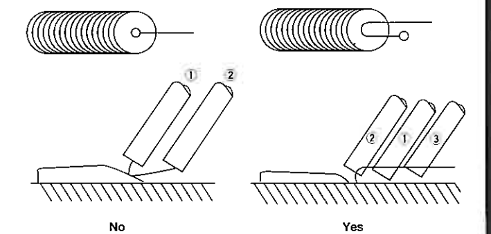
Fig.5 The backstep technique prevents porosity at the arc starting area of the weld bead
