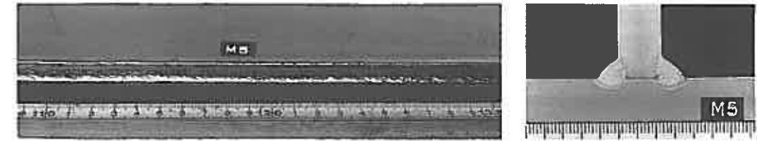
Fig.2 Bead appearance and cross-sectional view of a fillet weld (MX-200, 1.2mm φ, 280Amp. 28-32Volt, 50cm/min)
