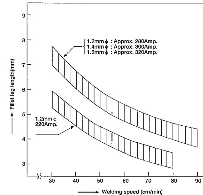
Fig.3 The relationship between welding speed and fillet leg length
