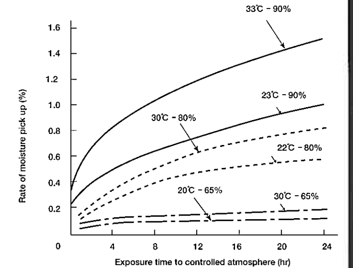
Fig.4 The moisture pick up vs. several temperatures and levels of humidity of the controlled testing atmosphere
