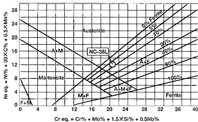
Fig.1 Schaeffler diagram
