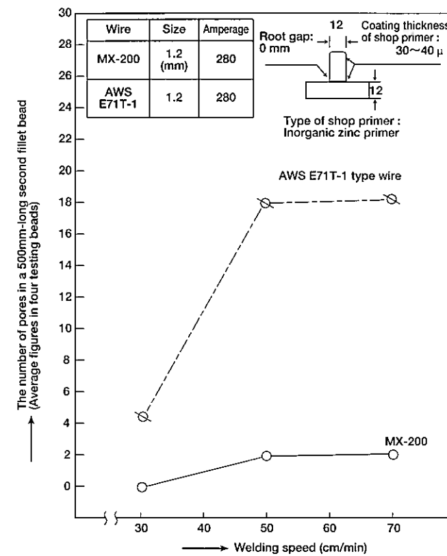
Fig.1 The results of testing the porosity susceptibility of flux-cored wires in fillet welding shop-primer-painted steel plates
