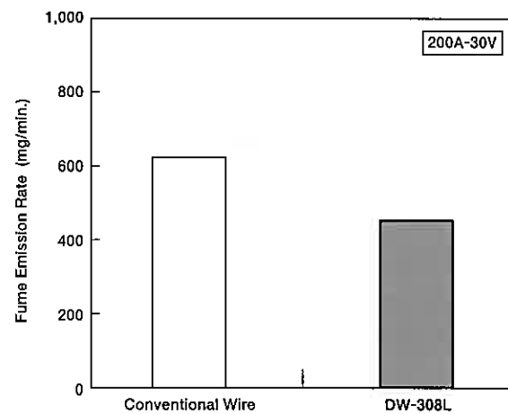
Fig.2 - A Comparison between DW-308L and a Conventional Flux Cored Wire on Fume Emission Rate (Wire Size: 1.2 mm φ, Shielding Gas: 100% CO 2 )
