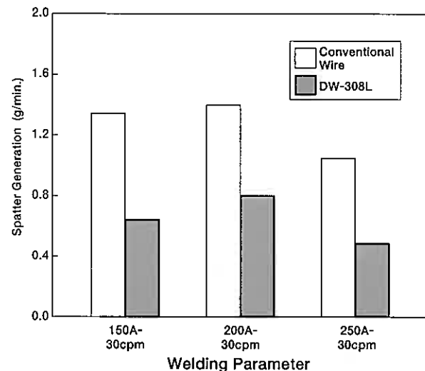
Fig.1 - A Comparison between DW-308L and a Conventional Flux Cored Wire on Spatter Generation (Wire Size: 1.2 mm φ, Shielding Gas: 100% CO 2 )
