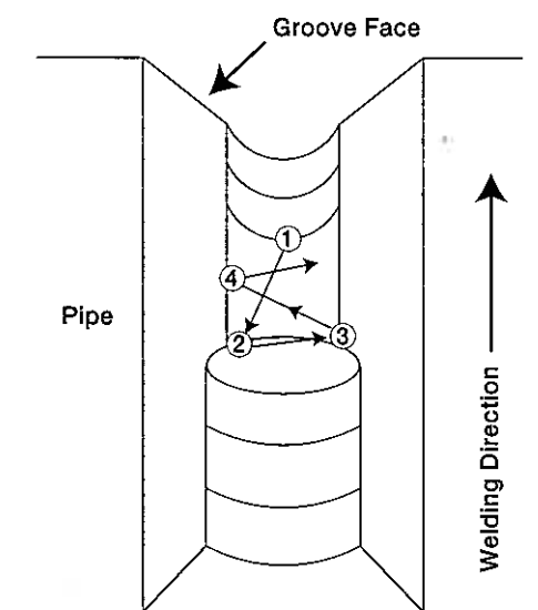
Fig.5 - The Backstep Technique in Vertical-Up Position Welding of Pipes ① Arc Start ② Backstep ③ Following Step ④ Following Step
