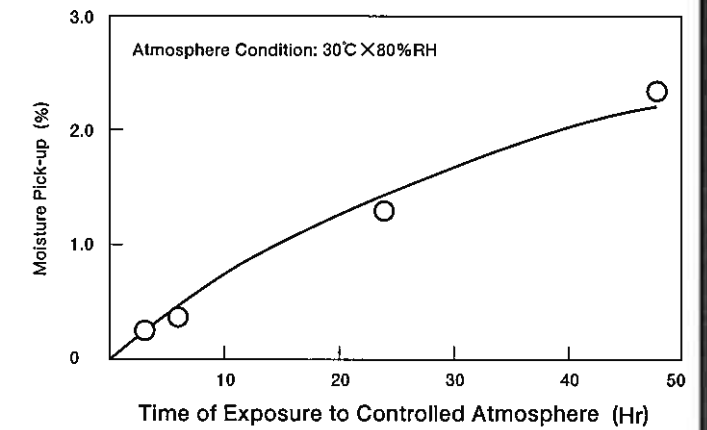
Fig.4 - The Relationship between Moisture Pick-Up and Time of Exposure to Controlled Atmosphere
