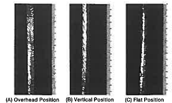
Fig.5 - MX-100T Bead Appearance on the Reverse Side of the Groove in the One-Side Root Pass Welding of Horizontally Fixed Pipes (Semi-Automatic, 1.2 mm φ Wire, 90 Amp.)
